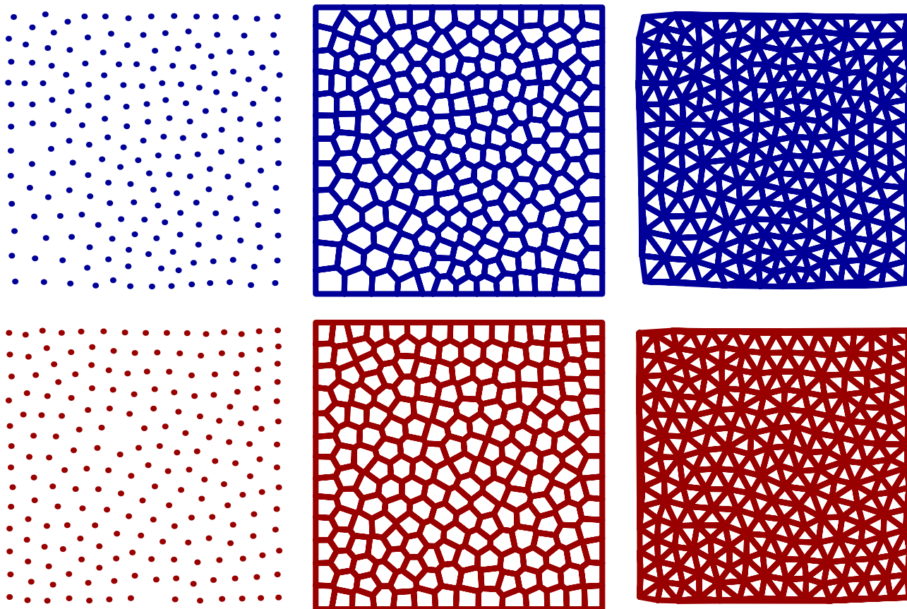
Figure 31.7 Poisson versus uniform randomization.
